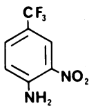
4-Amino-3-nitrobenzotrifluoride
