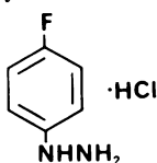
4-Fluorophenylhydrazine hydrochloride
